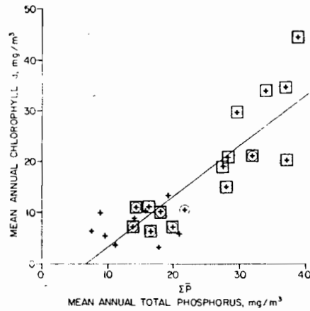
Fig. 1 (top). Relationship between mean annual concentrations of total phosphorus and chlorophyll a in lakes of the Experimental Lakes Area. All averages are weighted for morphometry of the lakes. Both fertilized and unfertilized lakes are included. (○) Data for fertilized lakes where nutrients supplied by fertilizer, precipitation, and runoff were deficient in nitrogen (N/P < 8 by weight). (□) Data for lakes where nutrients from the same three sources were deficient in carbon (C/P < 50 by weight). Points (+) without either circles or squares represent lakes where C/P and N/P ratios in inputs are either natural or higher than natural. The linear regression equation chlorophyll a = 0.987ΣP - 6.520 fits the points with the correlation coefficient r = .86 . Fig. 2 (middle). Mean annual total carbon and total phosphorus concentrations in fertilized lakes of the Experimental Lakes Area, illustrating how the carbon content of these lakes has increased because of addition of phosphorus. Total carbon includes seston, dissolved inorganic carbon, and methane, but excludes dissolved organic carbon (DOC). Concentrations of DOC have not changed as a consequence of eutrophication. (○) Data for lakes that received no carbon with fertilizer. (□) Data for lakes that received low fertilizations with sucrose (C/P ~ 6 by weight in lake 226, ~ 14 in lake 304, and ~ 85 in lake 226 southwest). Points without circles or squares represent lakes with either natural or higher than natural C/P inputs. The regression equation \Sigma C = 173.6\Sigma P + 420.3 fits the points with r = .83 . Fig. 3 (bottom). Mean annual concentrations of total nitrogen and total phosphorus in fertilized lakes, illustrating that the nitrogen content of a lake increases when phosphorus input is increased, even when little or no nitrogen is added with fertilizer. (○) Data for lake 261, which received only natural nitrogen. (□) Data for lakes 226 northeast and 227. The N/P in input to lake 226 northeast in 1973 to 1975 and lake 227 in 1975 was less than 8. Points without circles or squares represent lakes with N/P equal to or greater than the natural ratio. The regression equation \Sigma N = 30.9\Sigma P - 29.3 fits the points with r = .86 .
