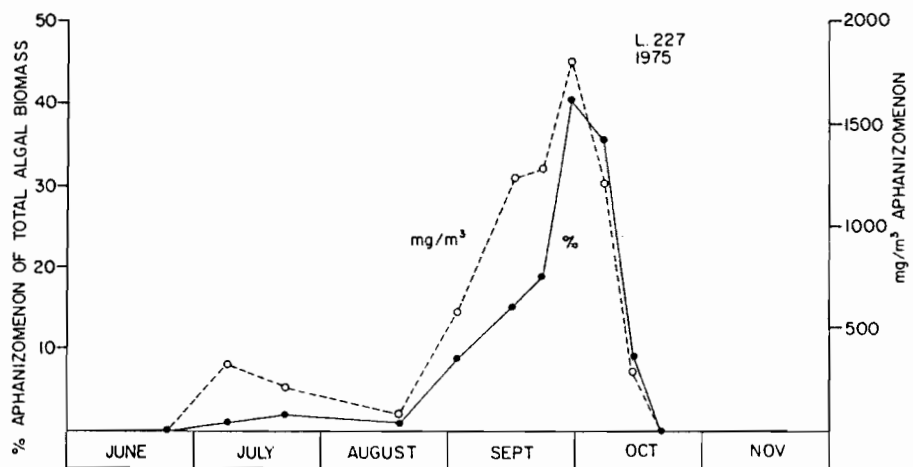
Fig. 4. Summer population of Aphanizomenon in lake 227 in 1975, after the N/P ratio in fertilizer had been cut back to 5 by weight. The genus had not been observed in quantifiable numbers in any of the six previous years, when an N/P ratio of 15 had been used in fertilizer. High fixation of atmospheric nitrogen accompanied the bloom of this species.
